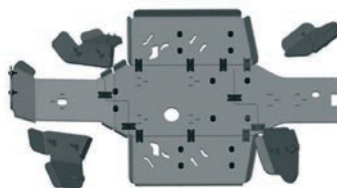
HDPE SKID PLATE ASSEMBLY (8 mm) - 2UP M01A05-C0403-001072
